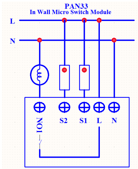
Fig 1. Assembling and wiring
