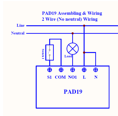
Fig 1. Assembling & Wiring
